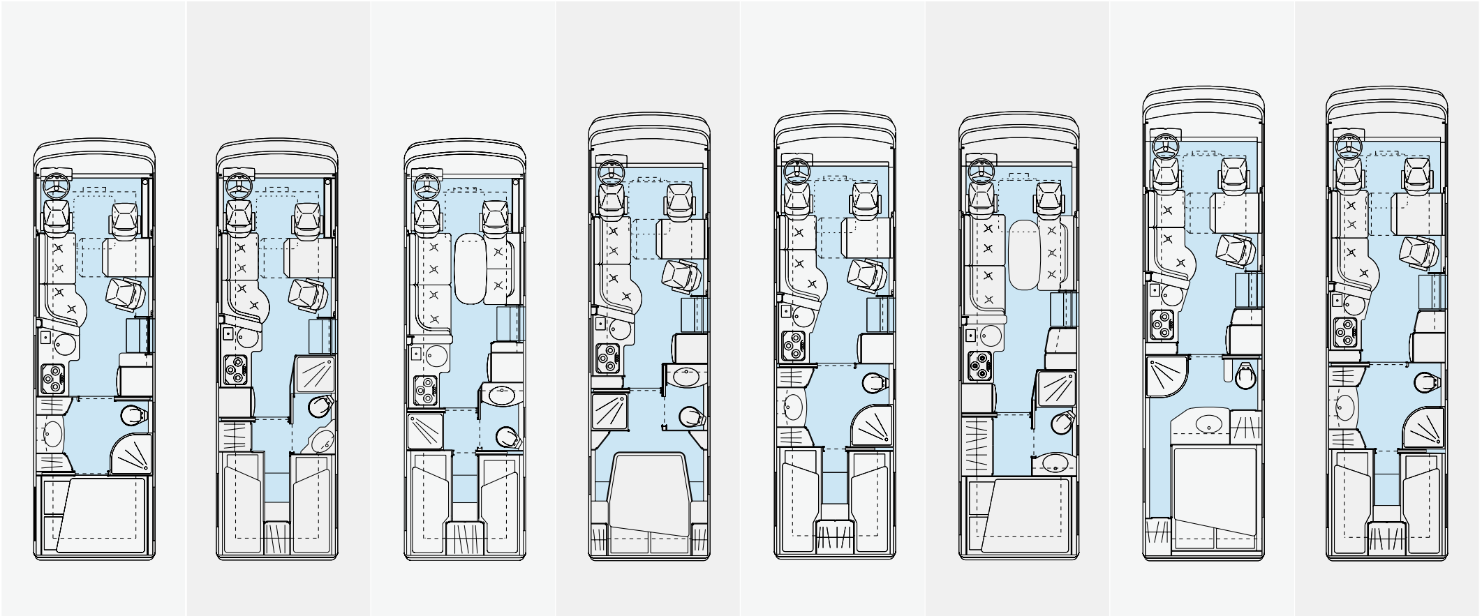
Star 800 / A Star 800 / B 2x rear end single beds Star 800 / C 2x rear end single beds Star 850 / A Smart garage Star 850 / B 2x rear end single beds Star 850 / C Star 900 / A Smart garage Star 900 / B 2x rear end single beds
